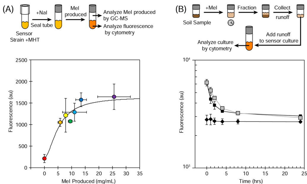
Figure 3. Yeast sensor detects MeI in MeI-producing cultures and MeI-contaminated soil. (A) The P_{8x.Cyc1}|P_{Adh1} sensor was used to screen a collection of methyl halide transferase (MHT) enzymes expressed from a plasmid cotransformed into S. cerevisiae . The MeI produced by each MHT as measured by GC-MS correlates with the fluorescence output of the sensor. The solid line shows a fit to a saturating function (Supporting Information). MHT homologues were derived from Batis maritima (violet), Burkholderia pseudomallei (dark blue), Burkholderia xenovorans (light blue), Vitis vinifera (green), Burkholderia thailandensis (yellow), Brassica rapa (orange), and Oryza sativa (red). Error bars are 1 standard deviation from three experiments performed on different days. (B) The experimental design for testing sensor activity in soil samples and the resulting data are shown. Tubes to which MeI was added at time 0 are shown as squares. Light squares represent tubes that were closed at time 0 and dark squares represent tubes that were left open to assess the impact of evaporation. Tubes to which only water was added to the soil are shown as black diamonds.
