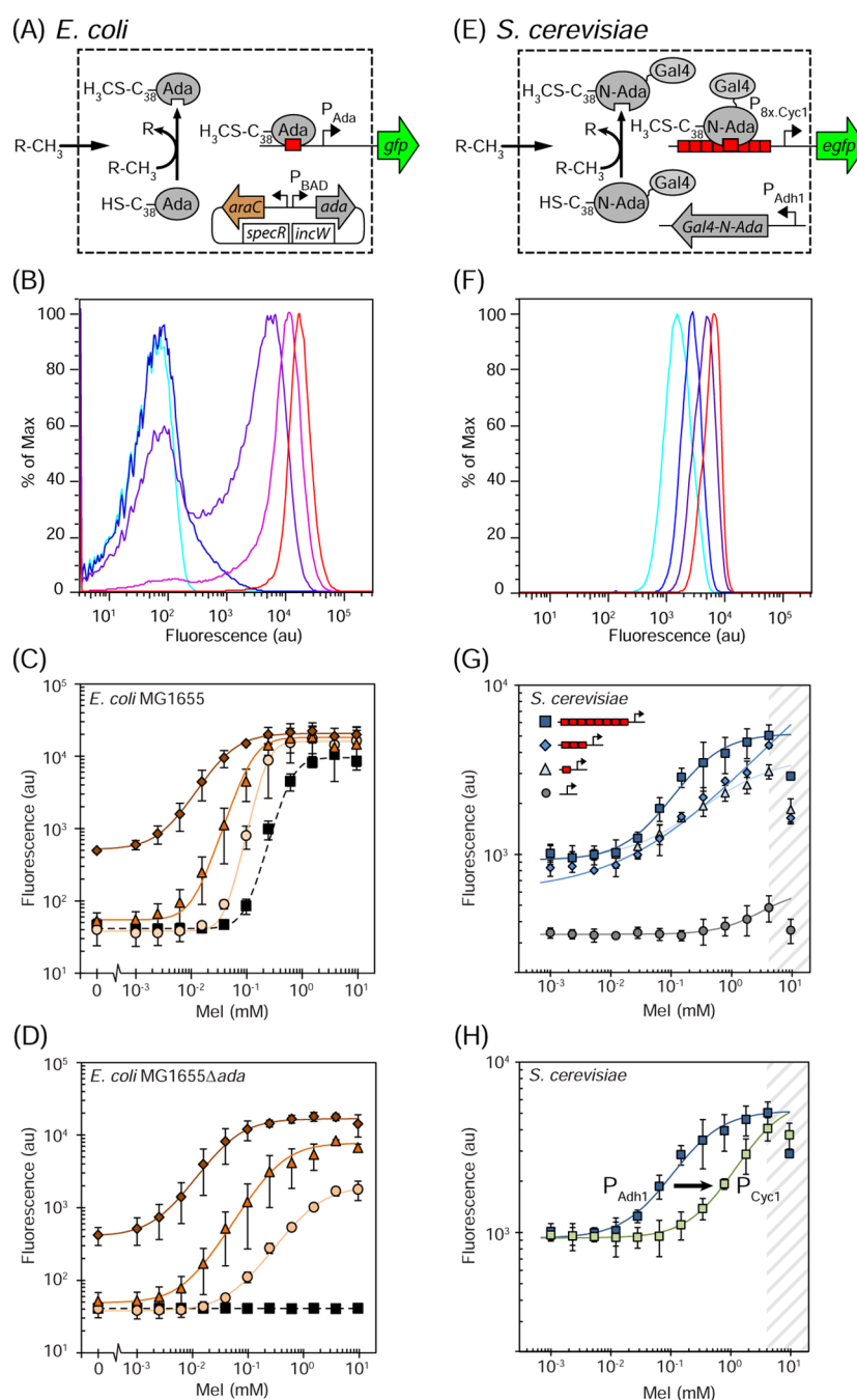
Figure 1. Mechanism and activity of E. coli and S. cerevisiae methylation sensors. (A) Diagram of the E. coli methylation sensor. The Ada protein is expressed from either the genome or a low-copy plasmid (inset in lower right). (B) Overlaid histograms show the induction of E. coli MG1655 carrying the plasmid pFM45. The line colors correspond to different concentrations of MeI: 0 (light blue), 98 μM (dark blue), 244 μM (violet), 610 μM (pink), and 3.8 mM (red). (C) Response functions for the methylation sensor are shown in E. coli MG1655. Solid lines are strains expressing inducible Ada from plasmid pFM141 with variable amounts of arabinose: 0 mM (circles), 1 mM (triangles), and 10 mM (diamonds). E. coli containing only the reporter plasmid pFM45 is shown for comparison (black squares, dashed line). (D) Response functions for the methylation sensor are shown for strain E. coli MG1655Δ ada . The same symbols and arabinose concentrations are used as in C. (E) Diagram of the S. cerevisiae methylation sensor. The sensor protein (Gal4-N-Ada) is expressed from the genome (inset in lower right). (F) The histogram shows the induction of S. cerevisiae carrying the P 8x.Cyc1 /P Adh1 methylation sensor. The line colors correspond to different concentrations of MeI: 0 (light blue), 148 μM (dark blue), 783 μM (violet), 9.5 mM (red). (G) Response functions of the methylation sensor in S. cerevisiae with variable number of operators upstream of the reporter promoter. Yeast sensor strains with promoter P 0x.Cyc1 (circles), P 1x.Cyc1 (triangles), P 3x.Cyc1 (diamonds), and P 8x.Cyc1 (squares) contain corresponding numbers of Ada operators upstream of reporter promoter P Cyc1 . The inset shows which symbols correspond to the number of operators in the promoter. The Gal4-N-Ada sensor protein in these strains is driven by the P Adh1 promoter. (H) Response functions of the methylation sensor in S. cerevisiae with Gal4-N-Ada expression driven by either the strong promoter P Adh1 (dark blue squares) or the weaker promoter P Cyc1 (light green squares). Both strains contain the EGFP reporter driven by promoter P 8x.Cyc1 . Diagonal gray dashes indicate MeI concentrations observed to be toxic (SI Figure S4). The P 8x.Cyc1 (squares) data is the same in both G and H for ease of comparison. Lines were generated by the sensor activation model described in the Supporting Information (SI) and are matched to their respective data by color. For all data, error bars represent one standard deviation from three independent experiments performed on different days.
