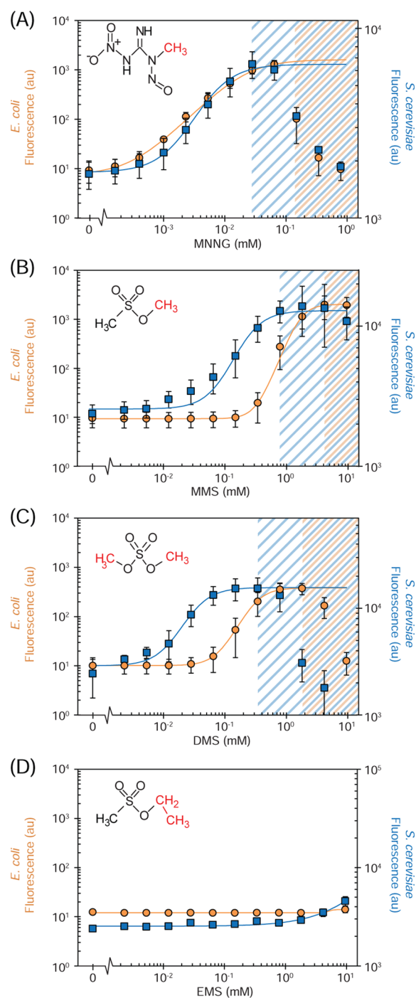
Figure 2. Response of the methylation sensors to S_N1 and S_N2 alkylating agents. E. coli MG1655 carrying plasmid pFM45 and S. cerevisiae sensor P_{8x,Cyc1}P_{Adh1} were exposed to (A) methylnitronitrosoguanidine (MNNG), (B) methyl methanesulfonate (MMS), (C) dimethyl sulfate (DMS), and (D) ethyl methanesulfonate (EMS). E. coli (orange circles) and S. cerevisiae (blue squares) data correspond to the left and right axes, respectively. Insets are the structures of the respective alkylating agents, with the donated alkyl group highlighted in red. Blue and orange shaded regions indicate concentrations of alkylating agent higher than the LD_{50} for S. cerevisiae and E. coli , respectively. The S. cerevisiae axis is scaled so that the highest and lowest values of the E. coli and S. cerevisiae curves are aligned for easier comparison. Toxicity of EMS was not measured. Error bars are one standard deviation from three independent experiments performed on different days.
